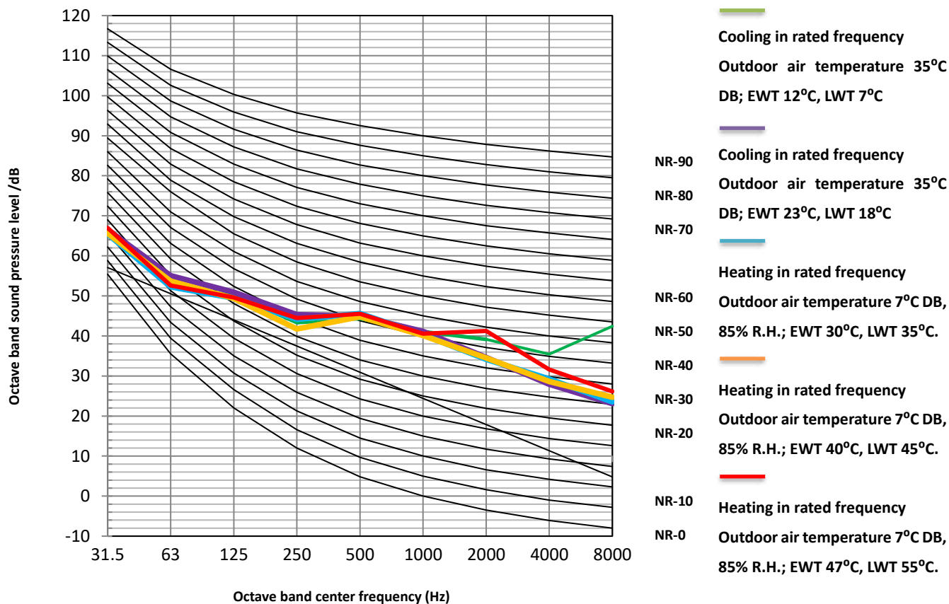
Figure 2-7.2: KHC-06RY1-B octave band levels
