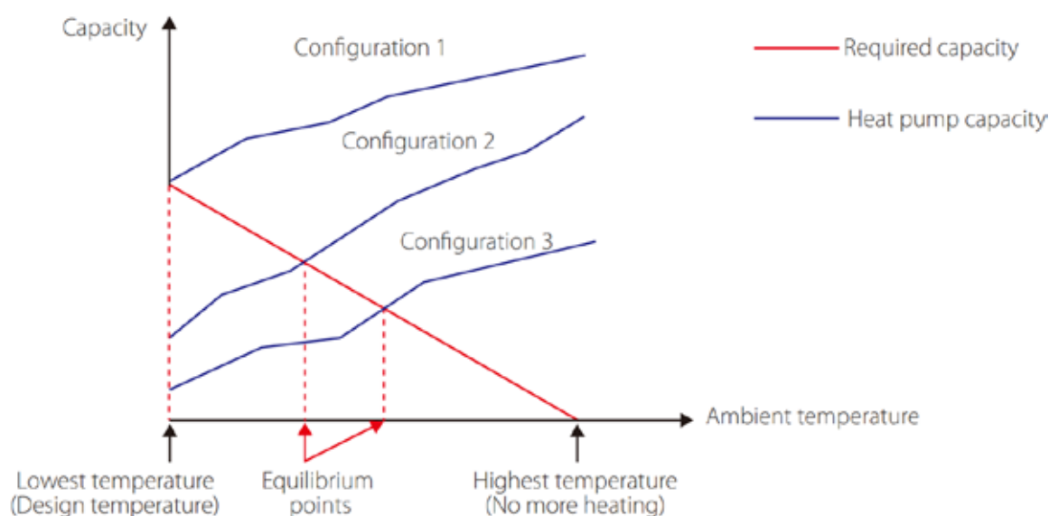
Figure 1-1.2: System configurations
