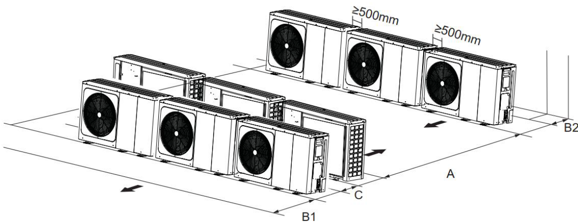
Figure 3-2.10: Multi-row installation
