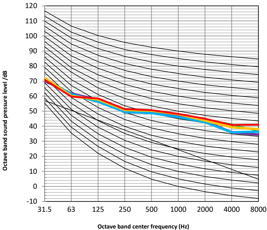
Figure 2-7.5: KHC-12RY3-B octave band levels
