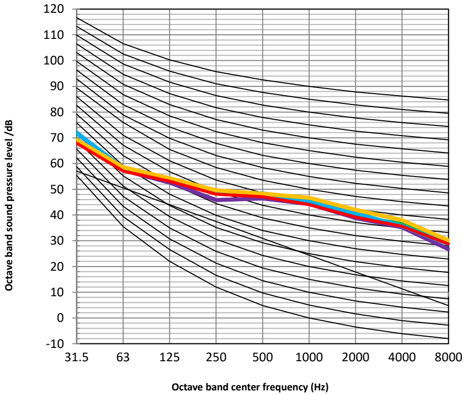
Figure 2-7.4: KHC-10RY3-B octave band levels
