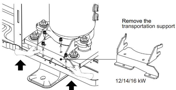
Figure 3-2.11: Remove the transportation support
